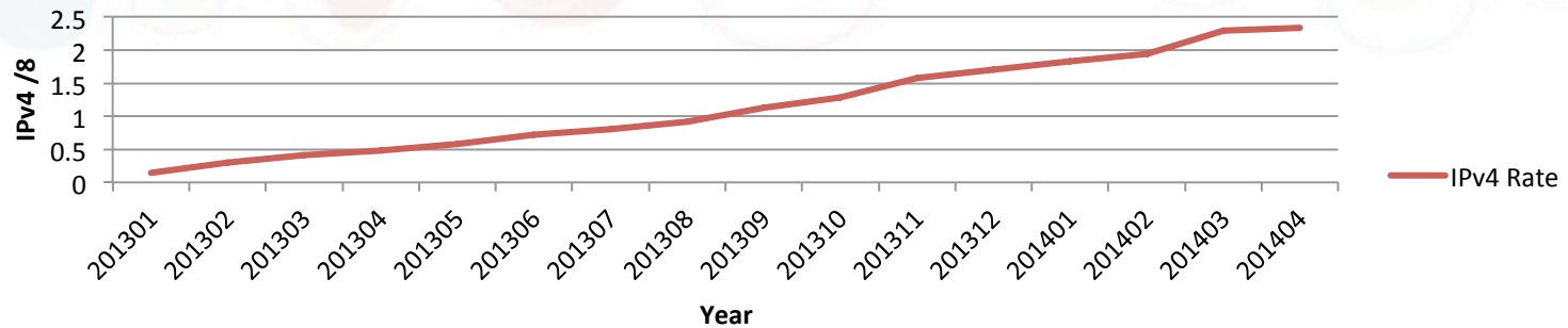
IPv4 /8 Accumulated
