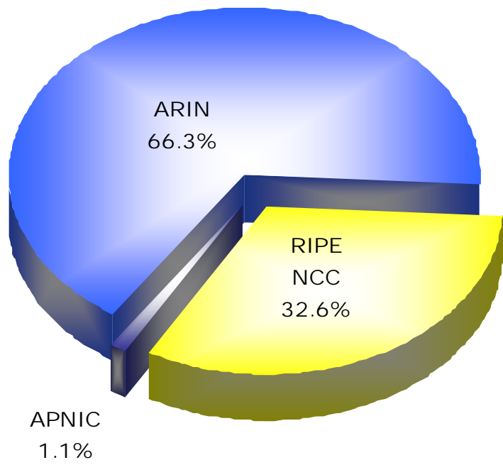
ASN
